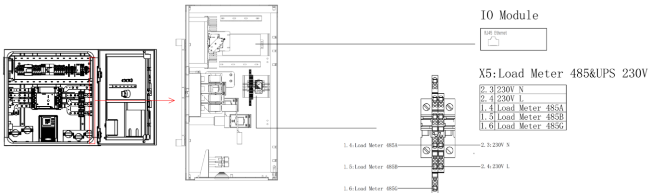
Figure 3-9 External ports
