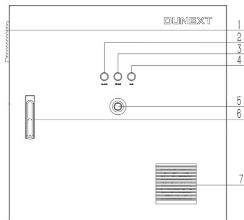
Figure 2-2 Front view of PCC
