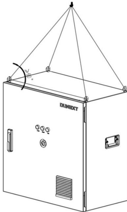
Figure 3-3 Hoisting angle ( \geq 60^\circ )
