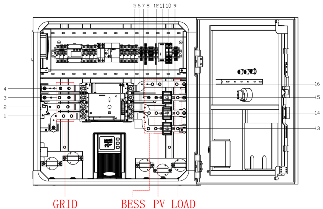
Figure 3-7 Wiring location in PCC
