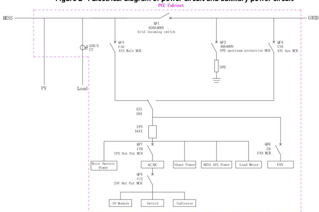
Figure 2-4 Electrical diagram of power circuit and auxiliary power circuit
