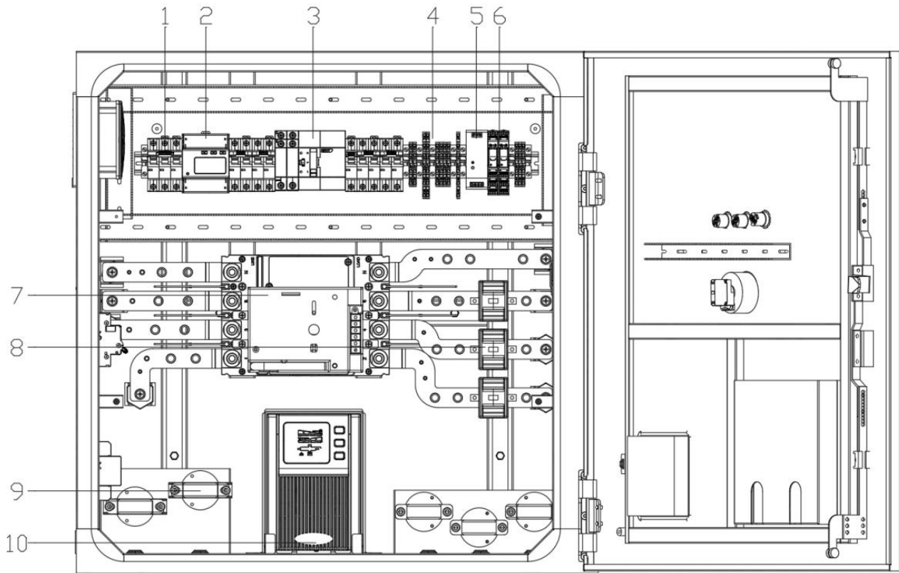
Figure 2-3 Structure design of PCC front view (door opened)
