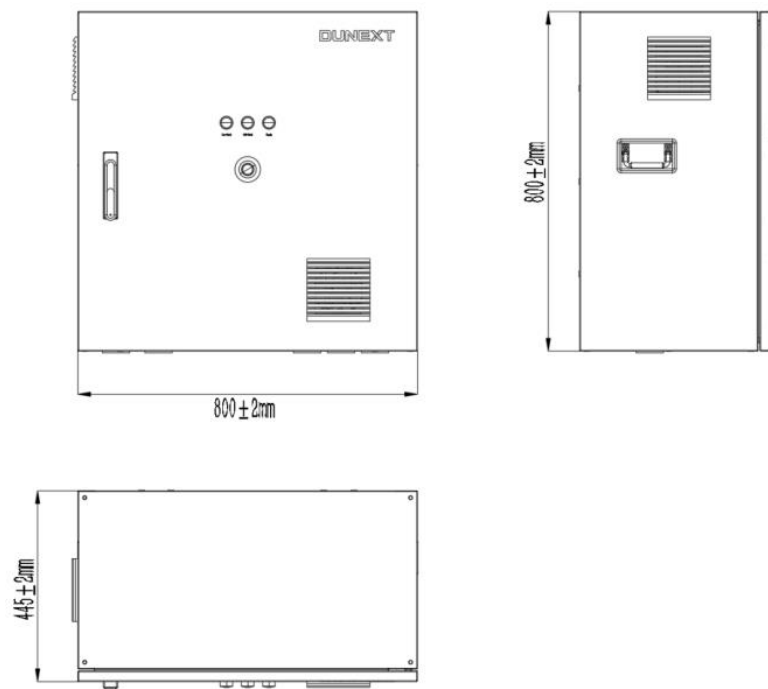
Figure 2-1 PCC dimensions (Unit: mm)
