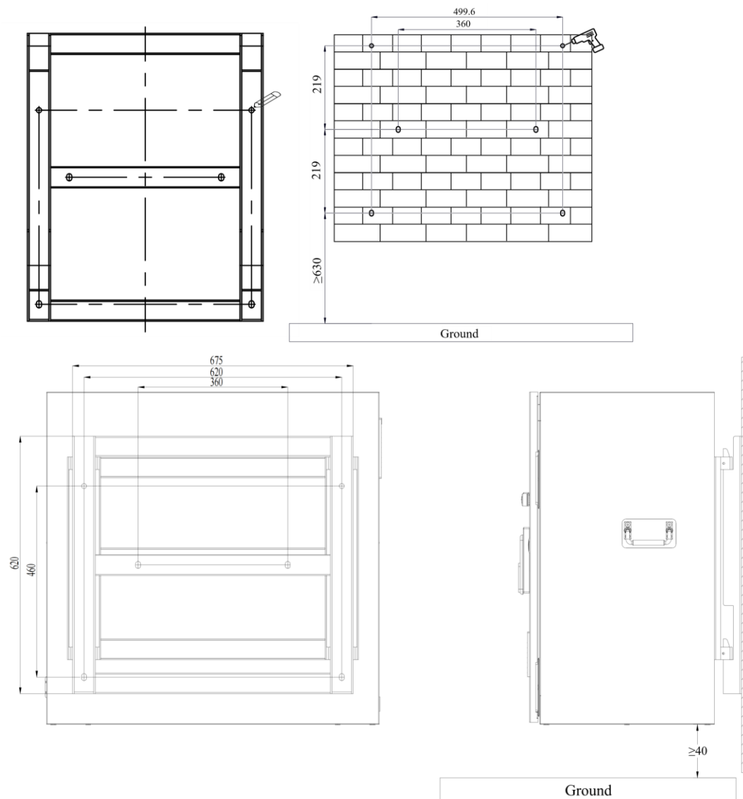
Figure 3-4 Wall-mounted installation (Unit: mm)
