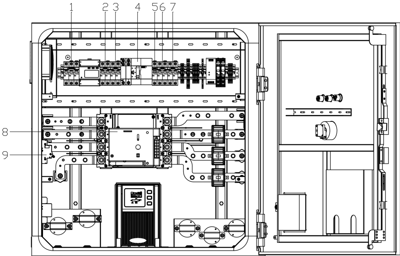
Figure 3-5 Switches in PCC
