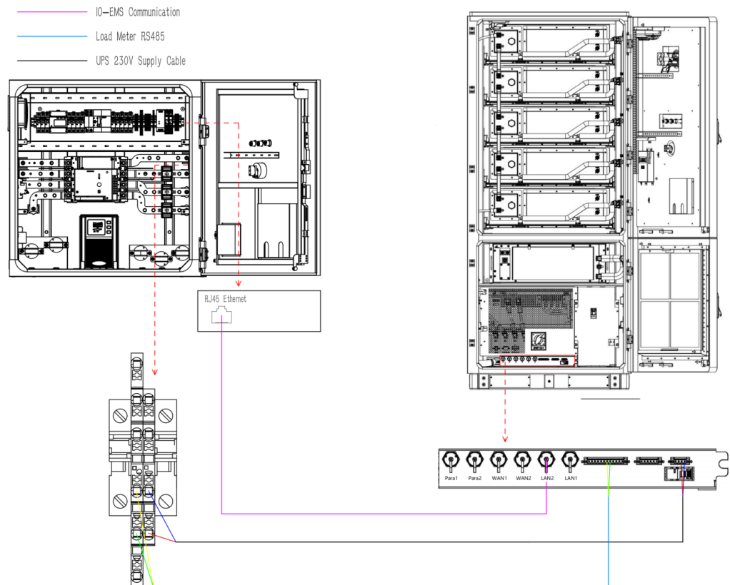
Figure 3-10 External ports connection diagram
