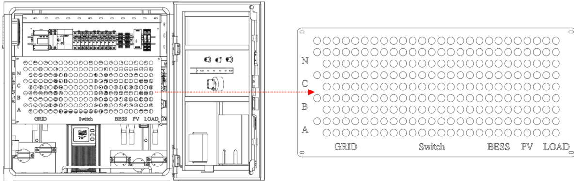
Figure 3-6 Silk-screen labels on the protective cover
