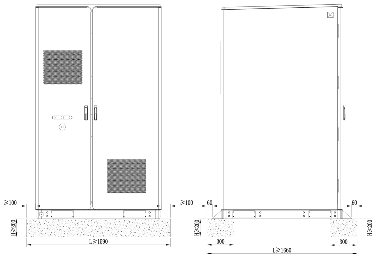
Figure 3-3 On-site foundation installation
